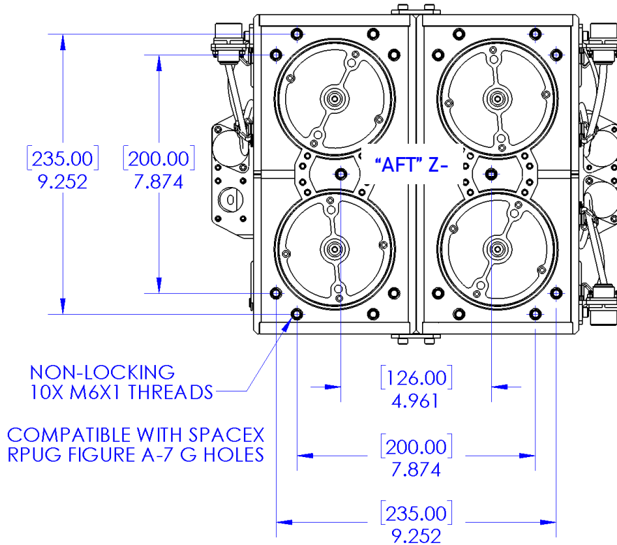
Figure 12: Quadpack Dispenser Aft Profile
