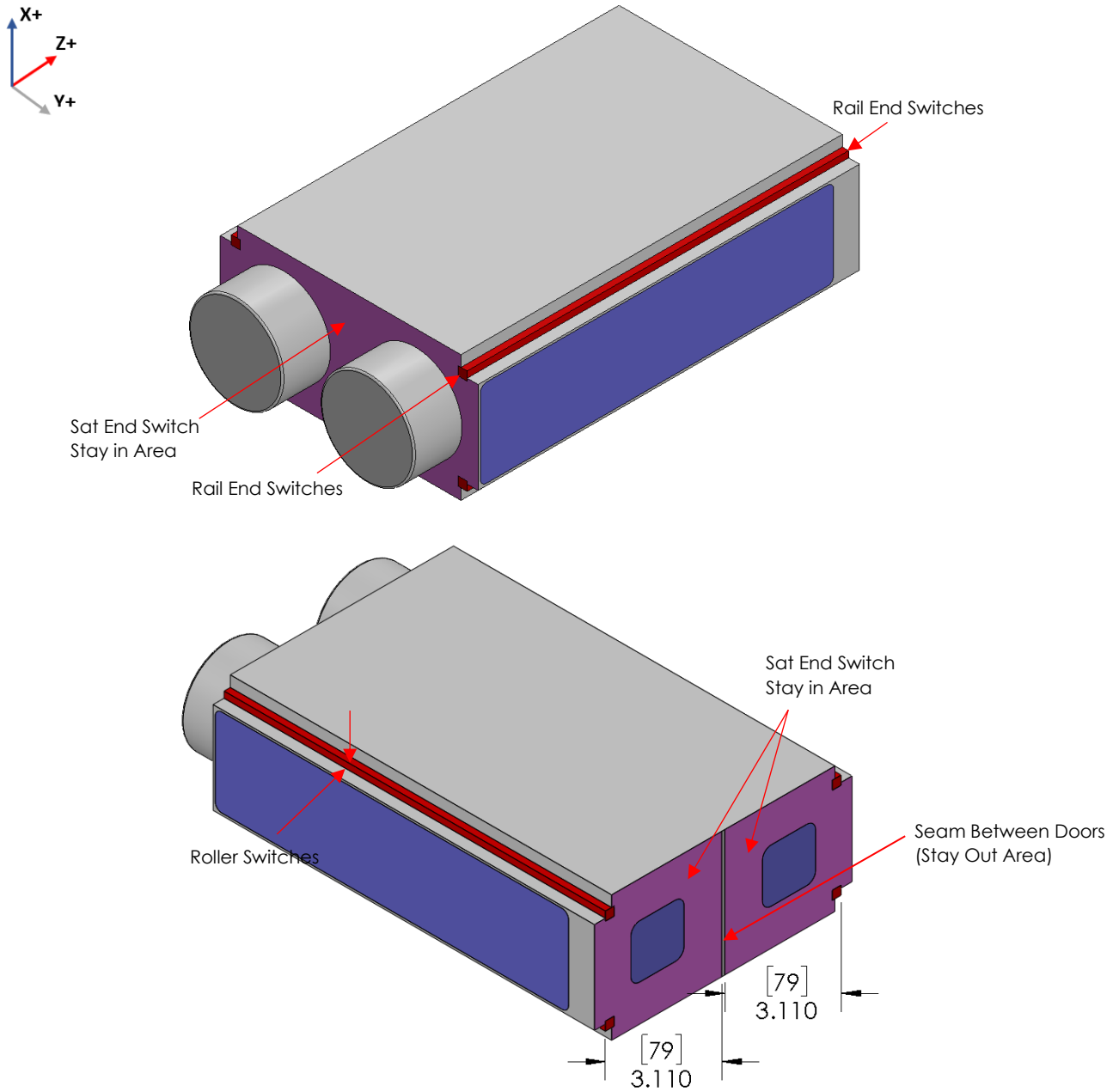
Figure 8: Switch general locations
