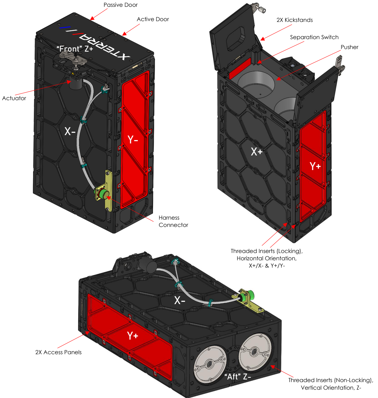
Figure 1: XCD 6U Configuration
